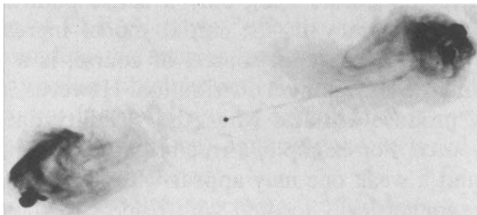
Figure: Three stages in the reduction of the observation of Cygnus A.
