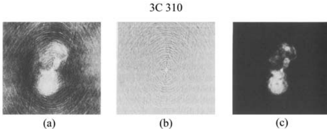
Figure: Images of the radio galaxy 3C10 from observations with the VLA.
